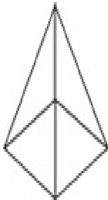
Square-based pyramid
