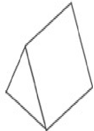
Triangular prism
