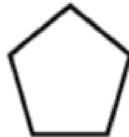
Pentagon 5 sides
