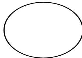
Full moon
