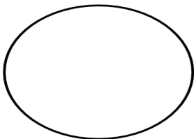
New Moon
