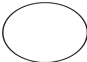
First Quarter
