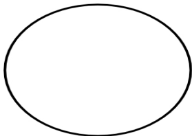
Waxing Crescent
