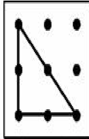
right-angled isosceles
