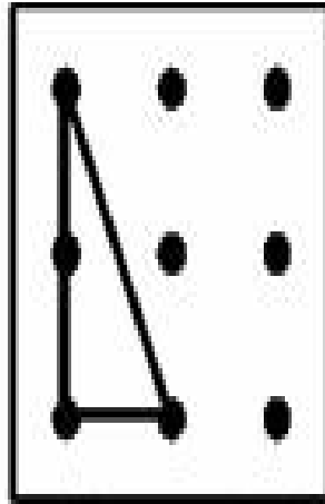
right-angled scalene
