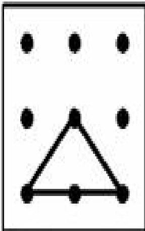
right-angled isosceles
