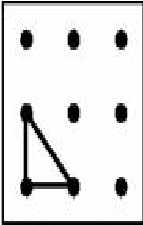
right-angled isosceles
