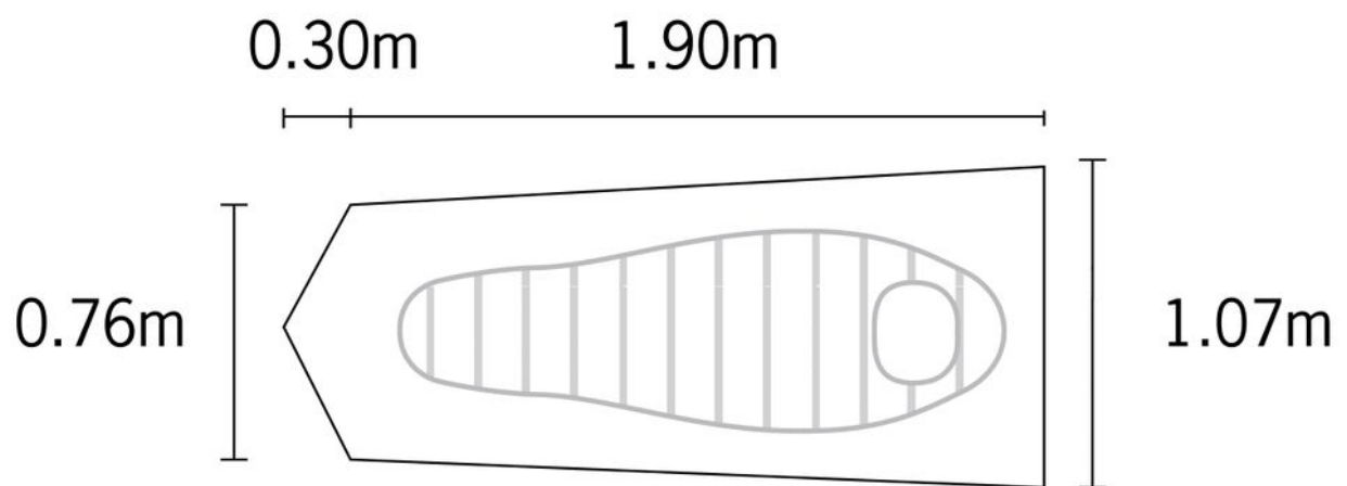
Fly Creek UL 1 Height Inside 0.97m
