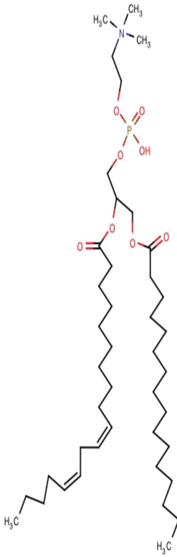
Phosphatidylcholine (PC)
