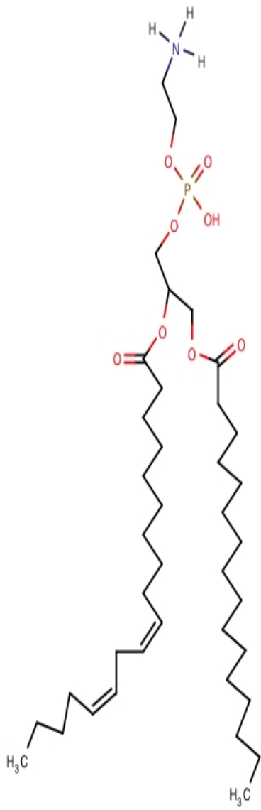
Phosphatidylethanolamine (PE)
