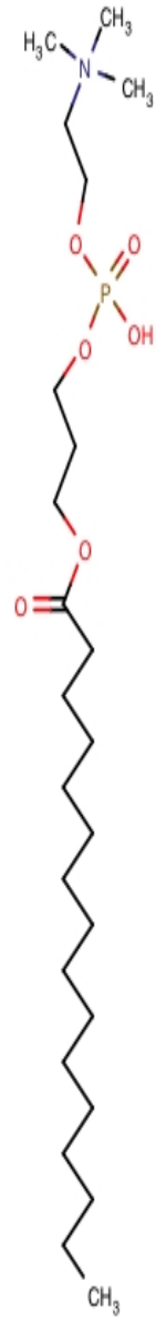
Lyso-phosphatidylcholine (LPC)
