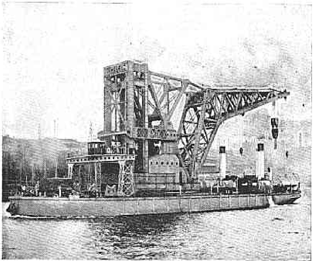
This Crane, built by Messrs. Cowans Sheldon and Co., Ltd., is capable of lifting and revolving with a load of 250 tons at 100 feet radius, and is the largest floating Crane in the world.
