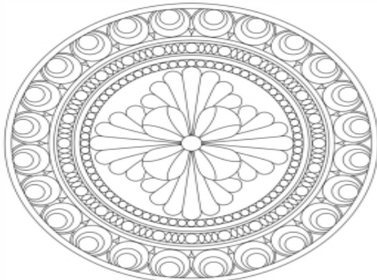
Four Fold
