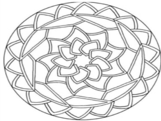
Nine Fold
