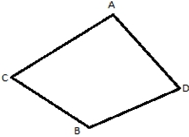
A convex quadrilateral
