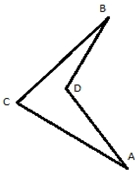
A concave quadrilateral
