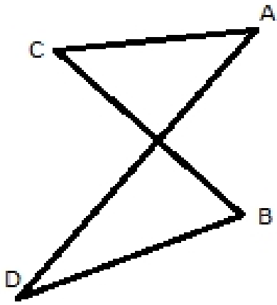
A crossed quadrilateral
