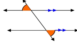
Alternate Exterior Angles Are Congruent
