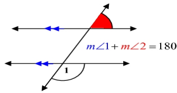
Same-Side Exterior Angles Are Supplementary
