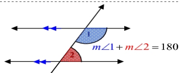
Same-Side Interior Angles Are Supplementary
