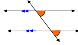
Corresponding Angles Are Congruent
