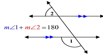
Same-Side Exterior Angles Are Supplementary
