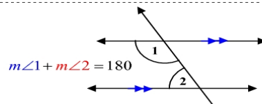
Same-Side Interior Angles Are Supplementary
