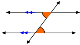
Alternate Interior Angles Are Congruent
