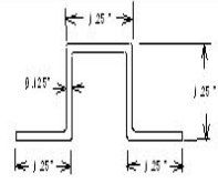
Section K-K (Longitudinal centerline floor support.)
