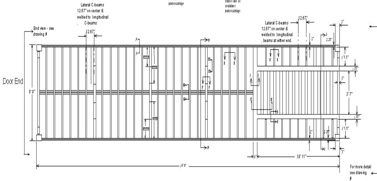
Section F-F
