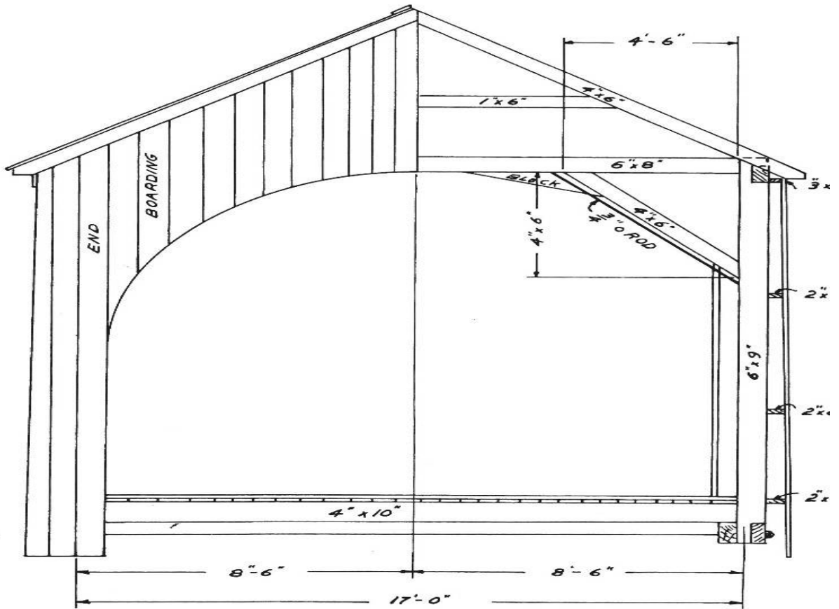
— END VIEW —
