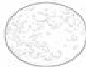
2. WAXING CRESCENT The moon is becoming visible from Earth, but we can only see a small piece of it. Draw a tiny crescent shape on the right, then shade the rest.
