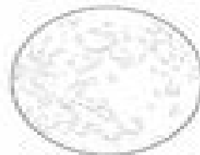
4. WANING GIBBOUS The moon appears almost full. Draw a crescent on the left, then shade it in.
