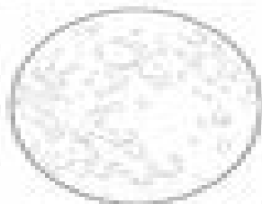
6. WAXING GIBBOUS The moon keeps its darken again. Draw a crescent on the right, then shade it in.
