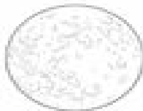
5. FULL MOON We can see the entire side of the moon. Leave the moon blank.
