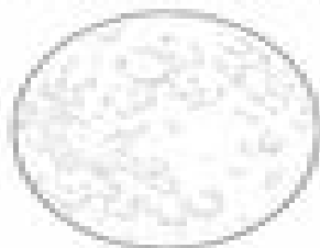
7. LAST QUARTER We can see a "half moon" again, with the visible side on the left. Shade in the right half.
