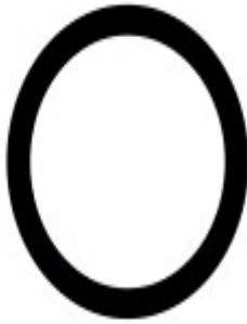
FULL MOON
