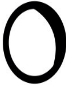
WANING GIBBOUS
