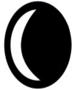
WANING CRESCENT
