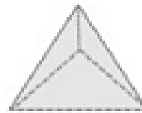
Triangular Pyramid
