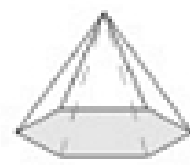
Hexagonal Pyramid
