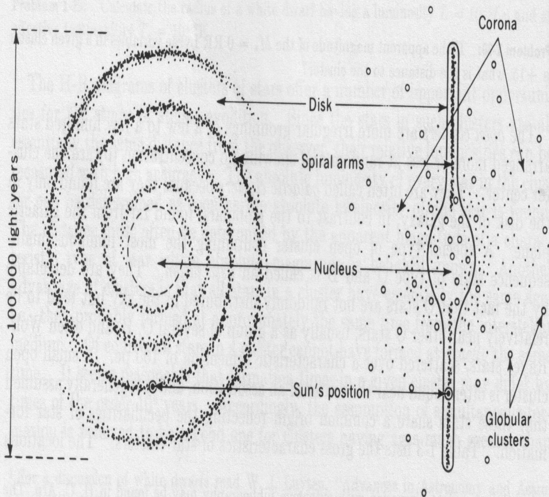
Fig. 1-13 Schematic representation of the galaxy. (G. Abell, Exploration of the Universe , Holt, Rinehart and Winston, Inc., New York, 1964.)
