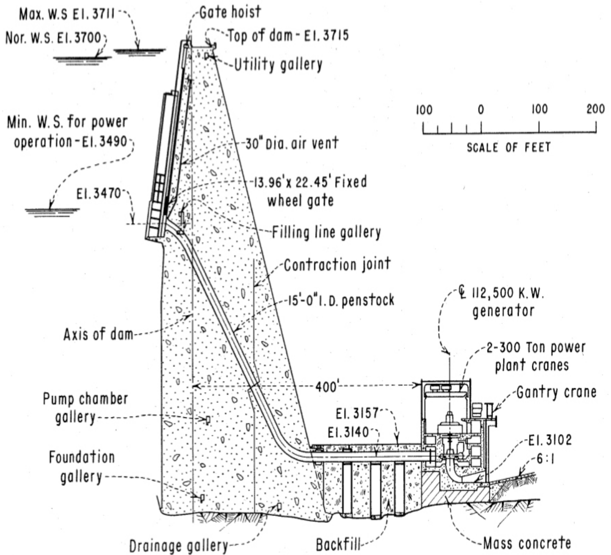
SECTION THRU PENSTOCK AND POWER PLANT
