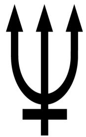
Neptune
