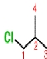
1-chloro-2-methyl propane
