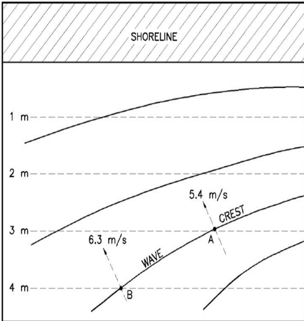
Figure II-3-3. Straight shore with all depth contours evenly spaced and parallel to the shoreline
