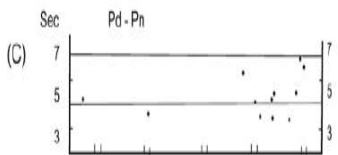
Figure 3. Precursory earthquakes of the 1943 eruption of Paricutin: (a) Earthquakes with magnitude M_s > 3 preceding the onset of the eruption. (b) Cumulative earthquake energy before the outburst, (c) Temporal change of seismic phases ( P_d - P_n ).
