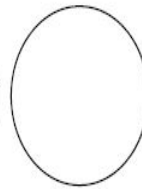
Full Moon
