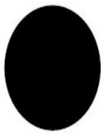
New Moon
