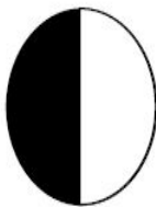
First Quarter
