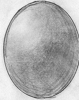
Sphere
