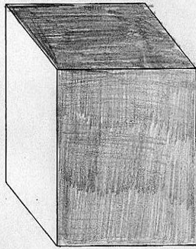
Cube
