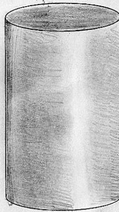
Cylinder
