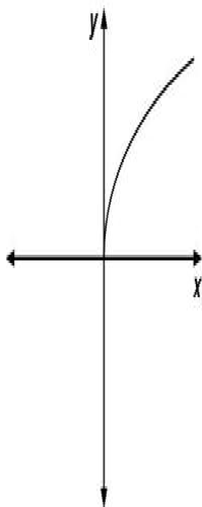
Square Root Pattern
