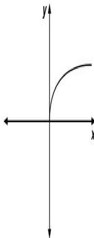
Fourth Root Pattern
