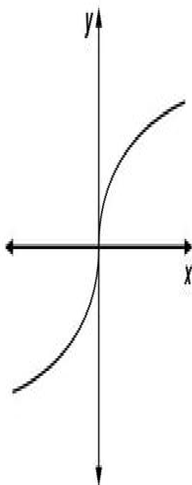
Cube Root Pattern
