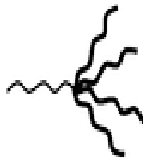
Palm-tree AB_n
