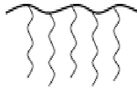
Comb polymer
