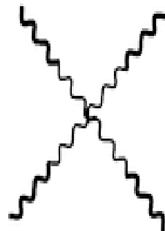
Star block AB_n
