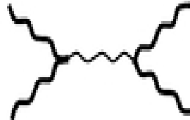
H-shaped B_2AB_2
