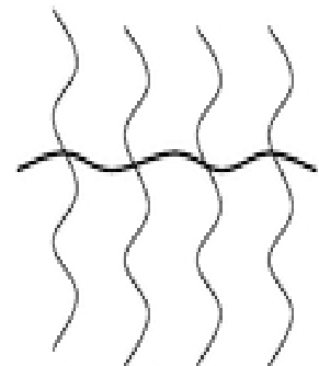
Brush polymer
