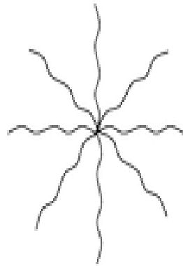
Star polymer
