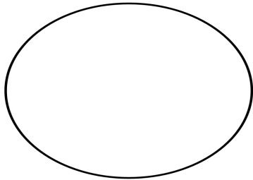
Full Moon
