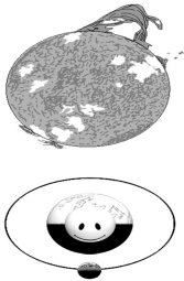
First Quarter
