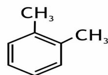
1,2-dimethylbenzene
