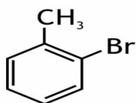
2-bromotoluene
