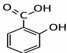
o-hydroxybenzoic acid
