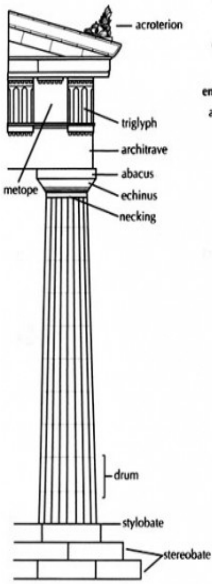
Doric order
