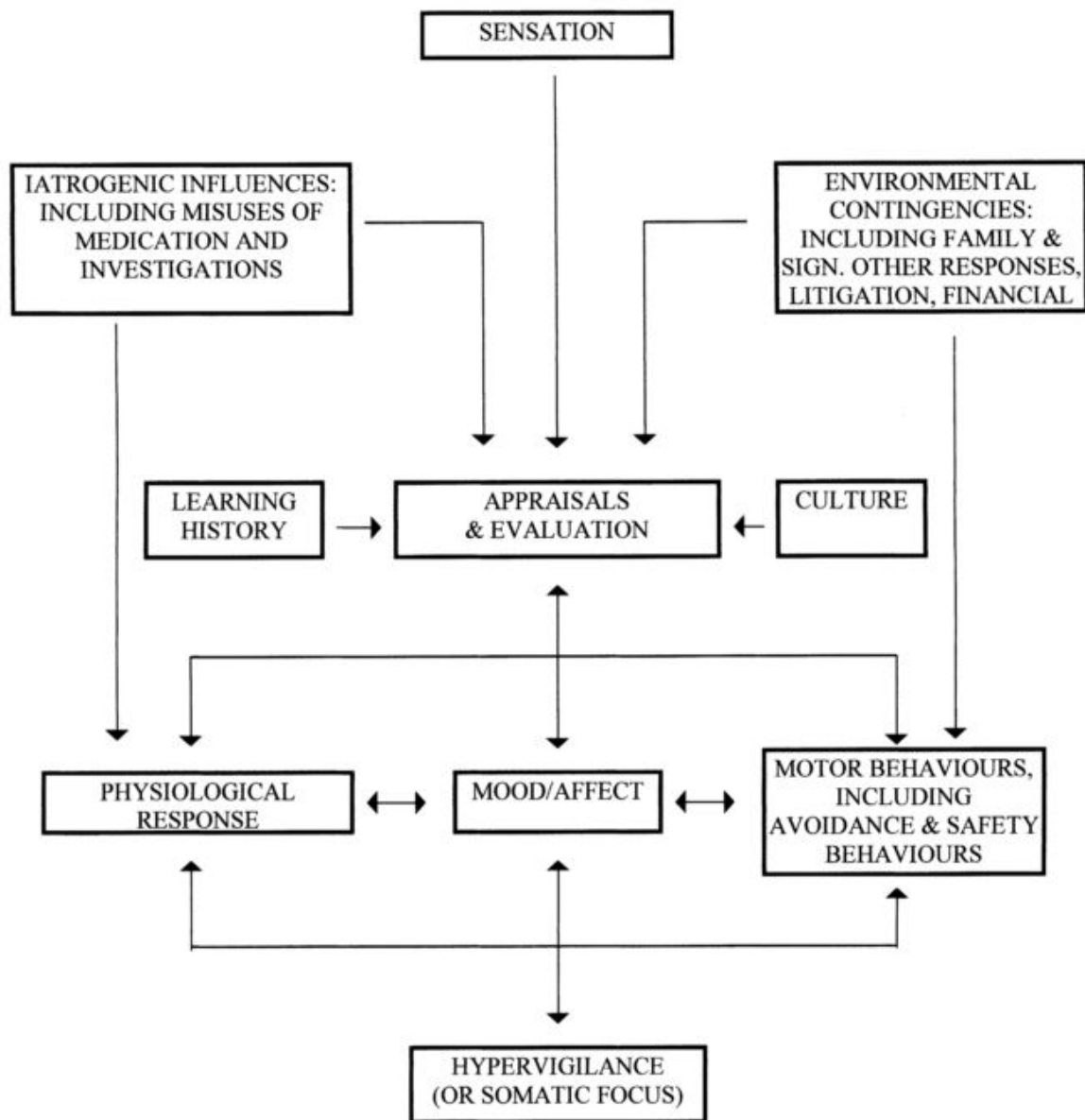
Fig. 1. The reformulated cognitive-behavioural model of chronic pain.
