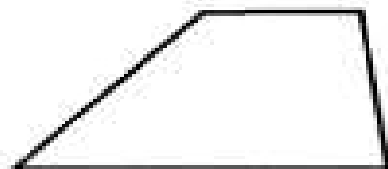
NO EQUAL SIDES NO EQUAL ANGLES TWO SIDES PARALLEL TRAPEZOID
