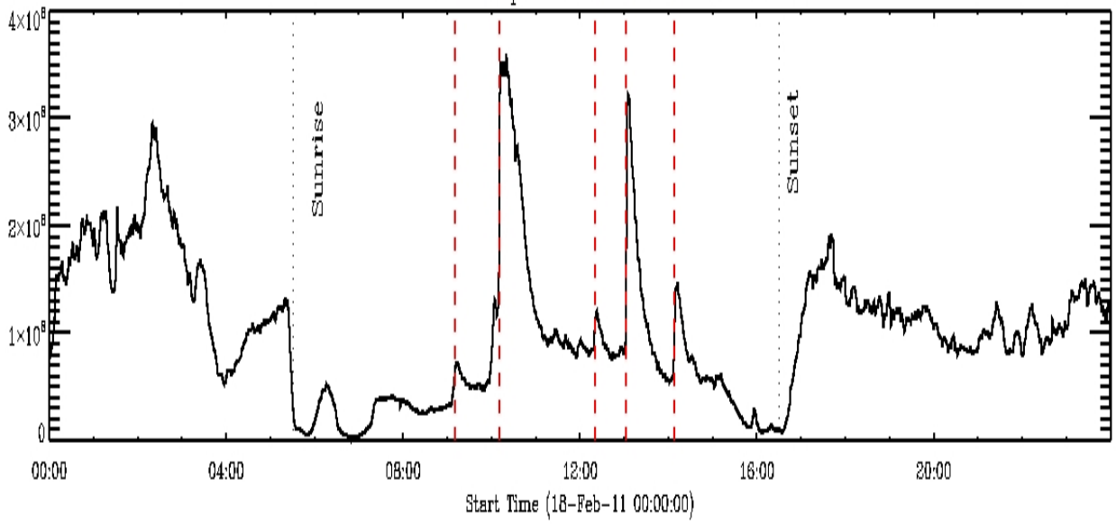
Sudden Ionospheric Disturbances - Austria
