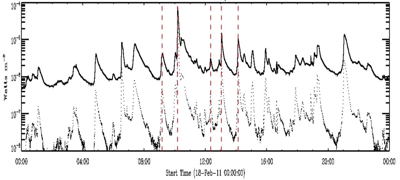
Sudden Ionospheric Disturbances - Austria
