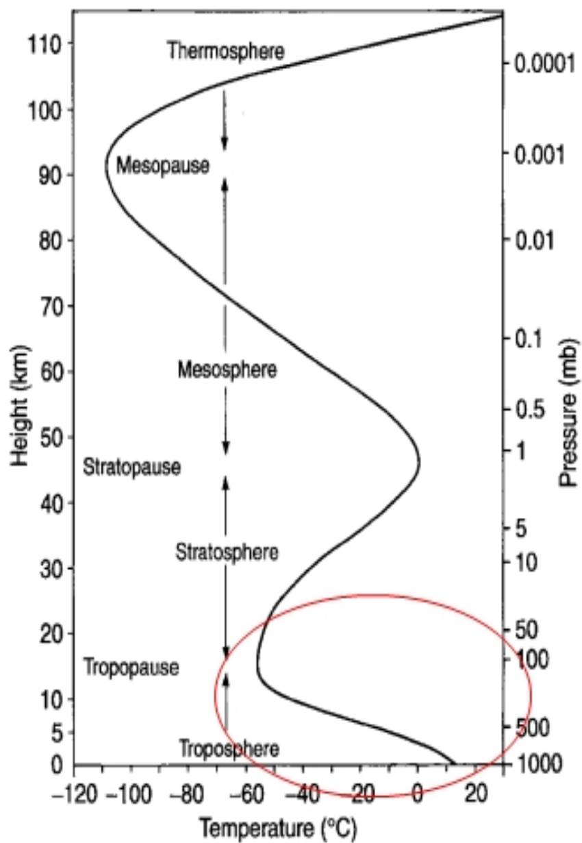
Fig. 1.3. Zonal mean vertical profile of temperature during June at 45°N.
